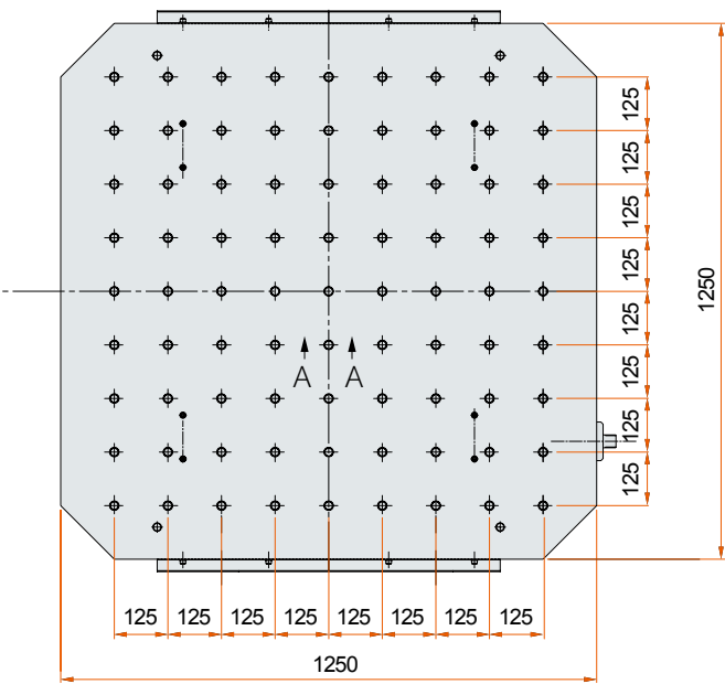
HCN-12800 1250 mm × 1250 mm tapped pallet
