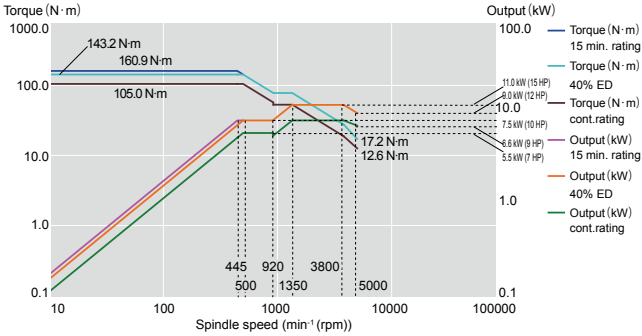
INTEGREX j-200, j-200S milling spindle
