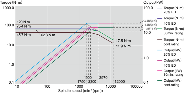
INTEGREX j-300, j-400 milling spindle
